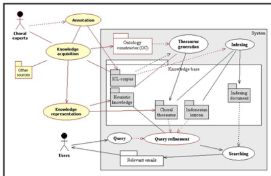
Figure 1. Use-Case Diagram of ontology based information retrieval system for Indonesian choral. (Notes: — association, —→ direct association, -.-→ dependency).
