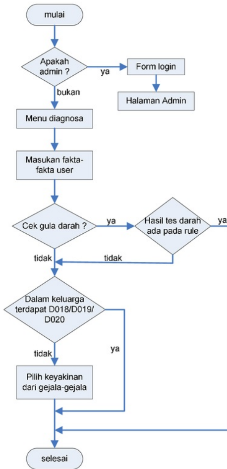
Gambar 1. Flowchart proses program
