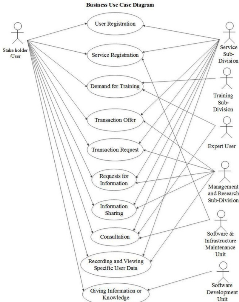
Figure 4: IAIS Business Use Case Diagram
